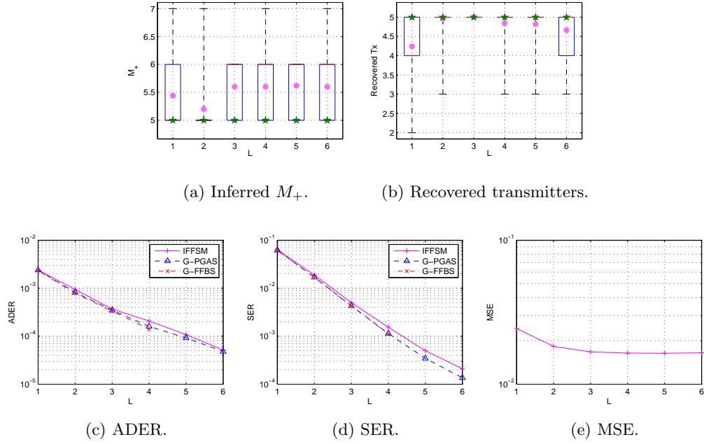
Figure 6.13: IFFSM results for different values of L .
