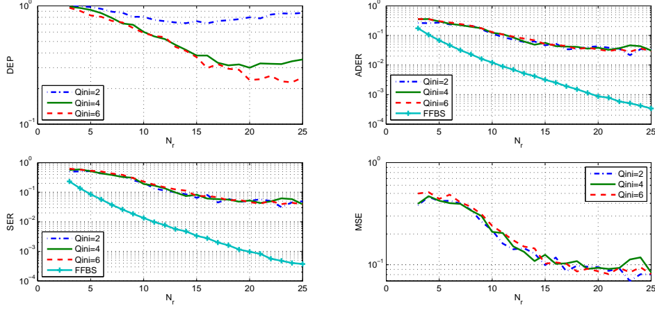
Figure 6.4: IFUHMM results for the Scenario C ( L = 2 , N_t = 3 and \text{SNR} = 0 dB).
