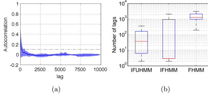
Figure 5.1: Autocorrelation plots for the small scale experiment. (a) Autocorrelation plot for the IFUHMM. (b) Number of samples for the autocorrelation to fall below 0.1.
