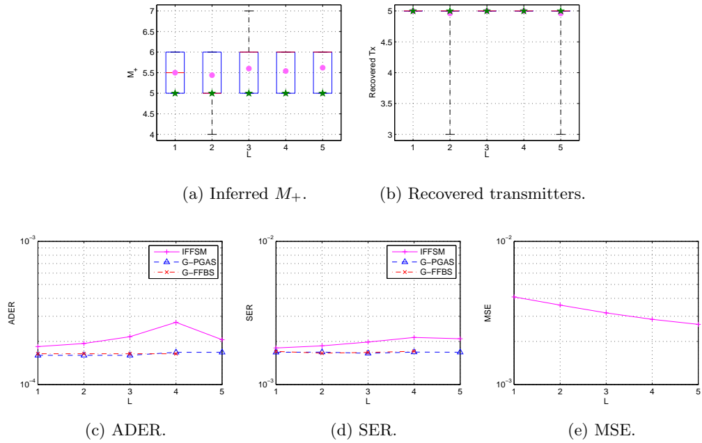
Figure 6.11: IFFSM results for different channel lengths ( L_{\text{true}} = 1 ).
