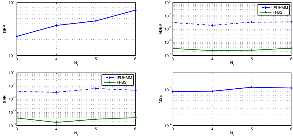
Figure 6.5: IFUHMM results for the Scenario D ( L = 2 , N_r = 25 and \text{SNR} = 0 dB).
