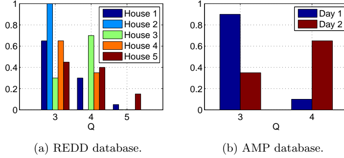
Figure 5.4: Histogram of the inferred values of Q under the IFUHMM.
