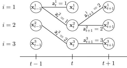
Figure 4.5: Example of the connection of particles in PGAS. We represent P = 3 particles \mathbf{x}_\tau^i for \tau = \{t-1, t, t+1\} . The index \mathbf{a}_\tau^i denotes the ancestor particle of \mathbf{x}_\tau^i . It can be seen that, e.g., the trajectories \mathbf{x}_{1:t+1}^1 and \mathbf{x}_{1:t+1}^2 only differ at time instant t+1 .
